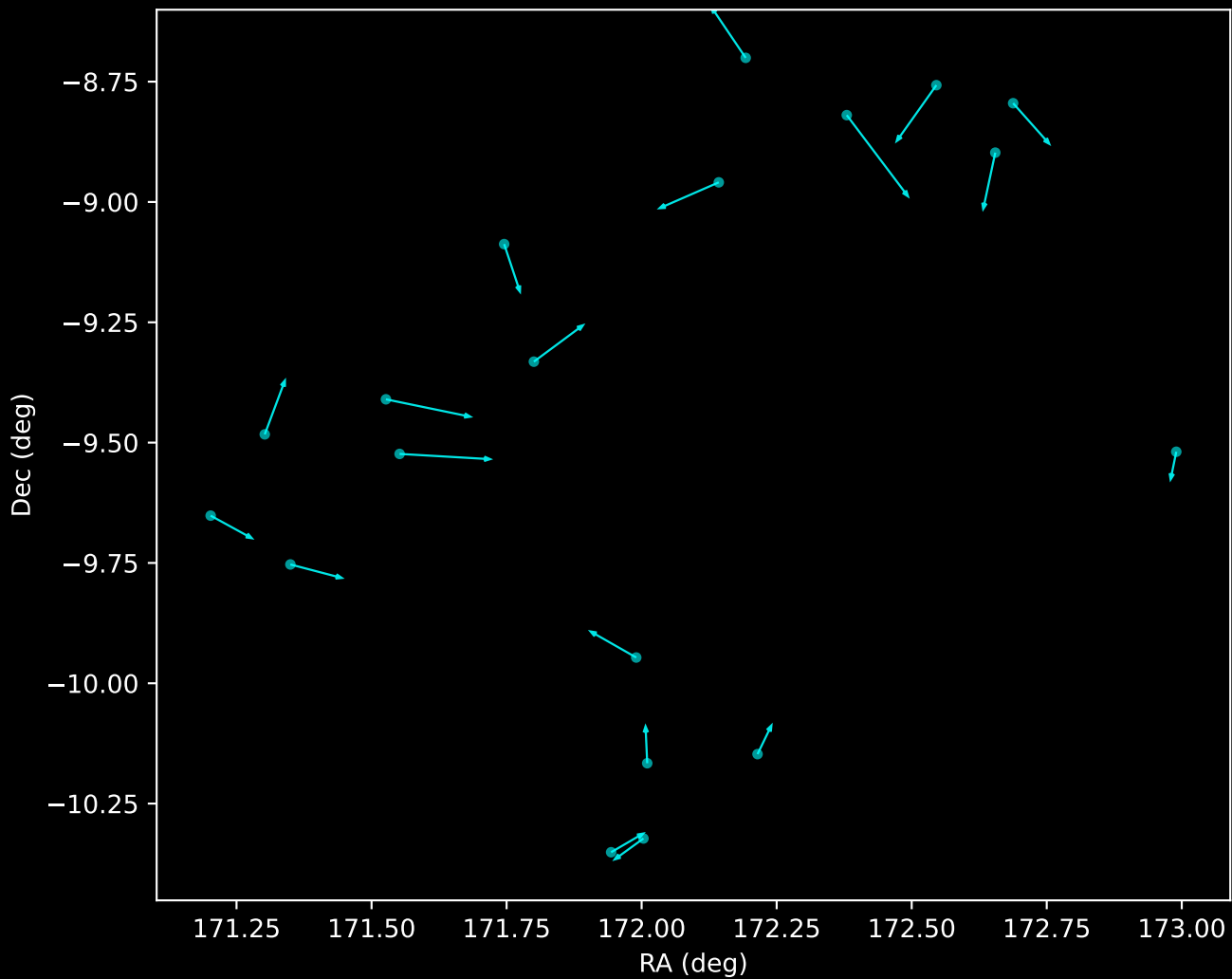
GALAH DR4 Noise Stream Proper Motion Vectors (n=19)
