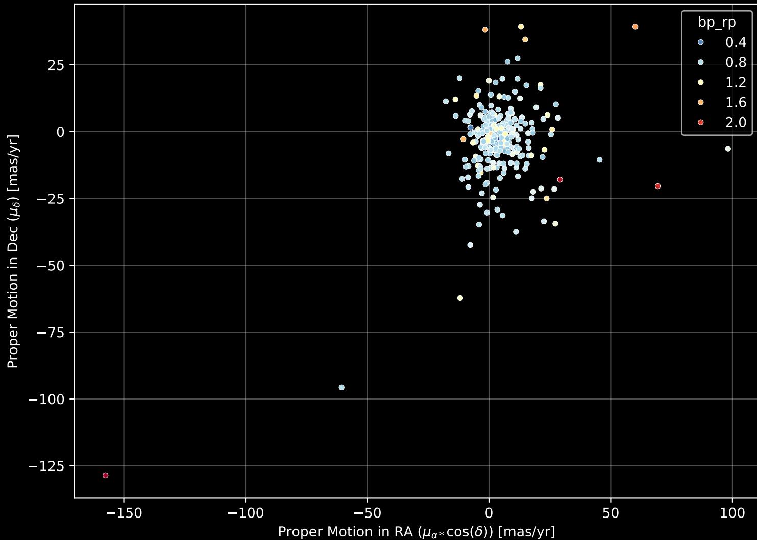
GALAH DR4 Field: [841] Proper Motion Diagram (n= 284)
