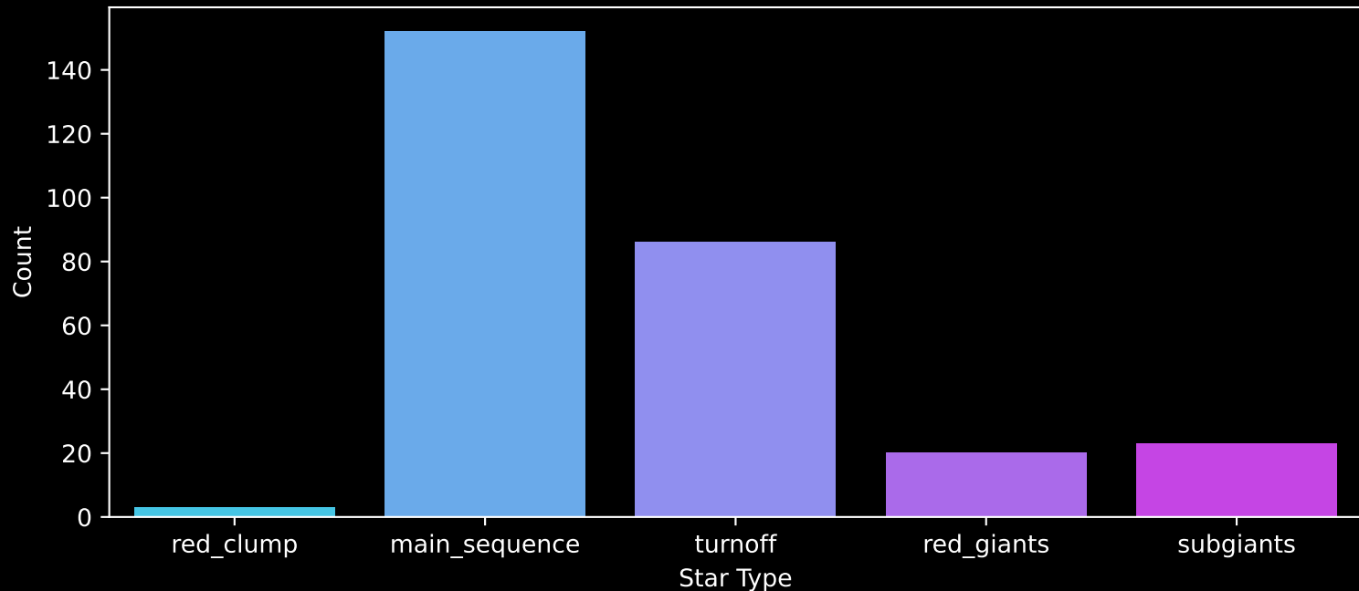
GALAH DR4 Field: [841] Count plot of Star Type
