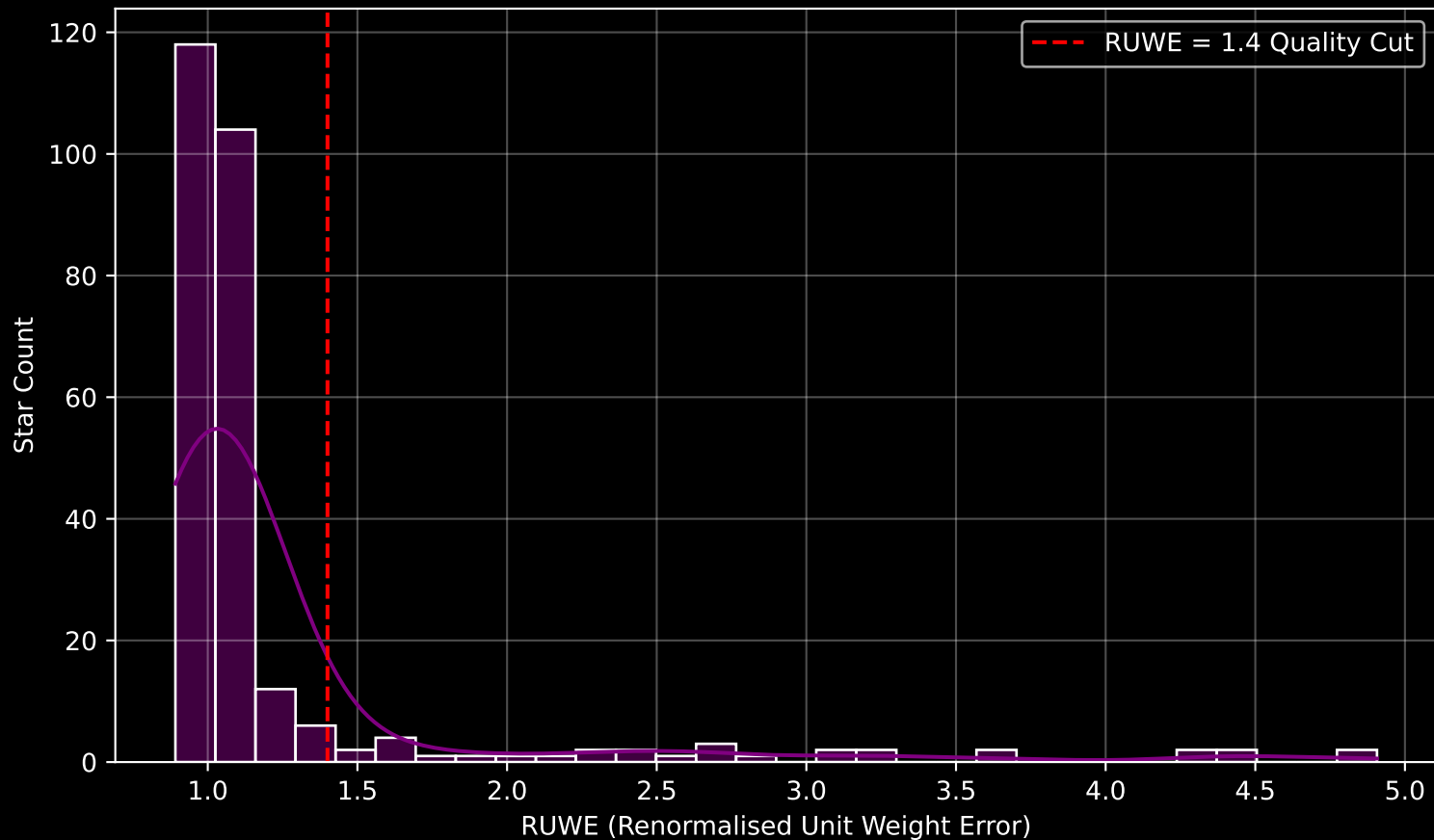
GALAH DR4 Field [841] RUWE Distribution (n= 271)
