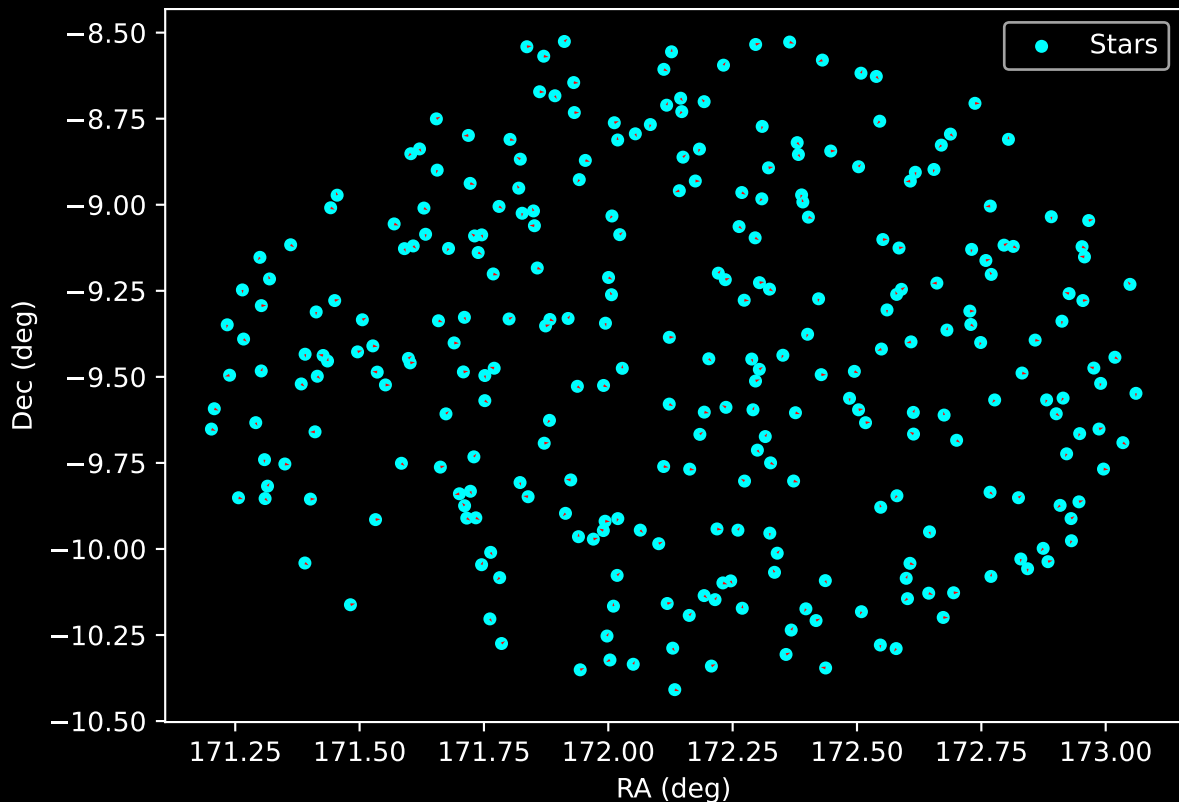
GALAH DR4 Field: [841] Proper Motion Vectors for Gaia Star Field (n= 284)
